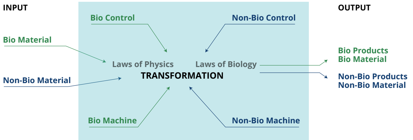
Figure 4.2 Classification of steps in the process chain. (T. Tolio G. Trotta, 3rd ManuFUTURE BIOINTELLIGENT MANUFACTURING plenary meeting)
